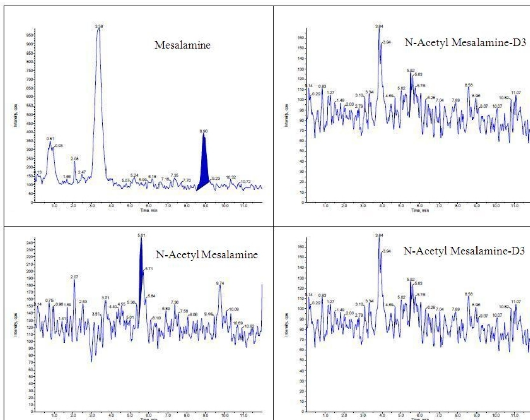
Fig. 4. Chromatogram of blank human plasma
