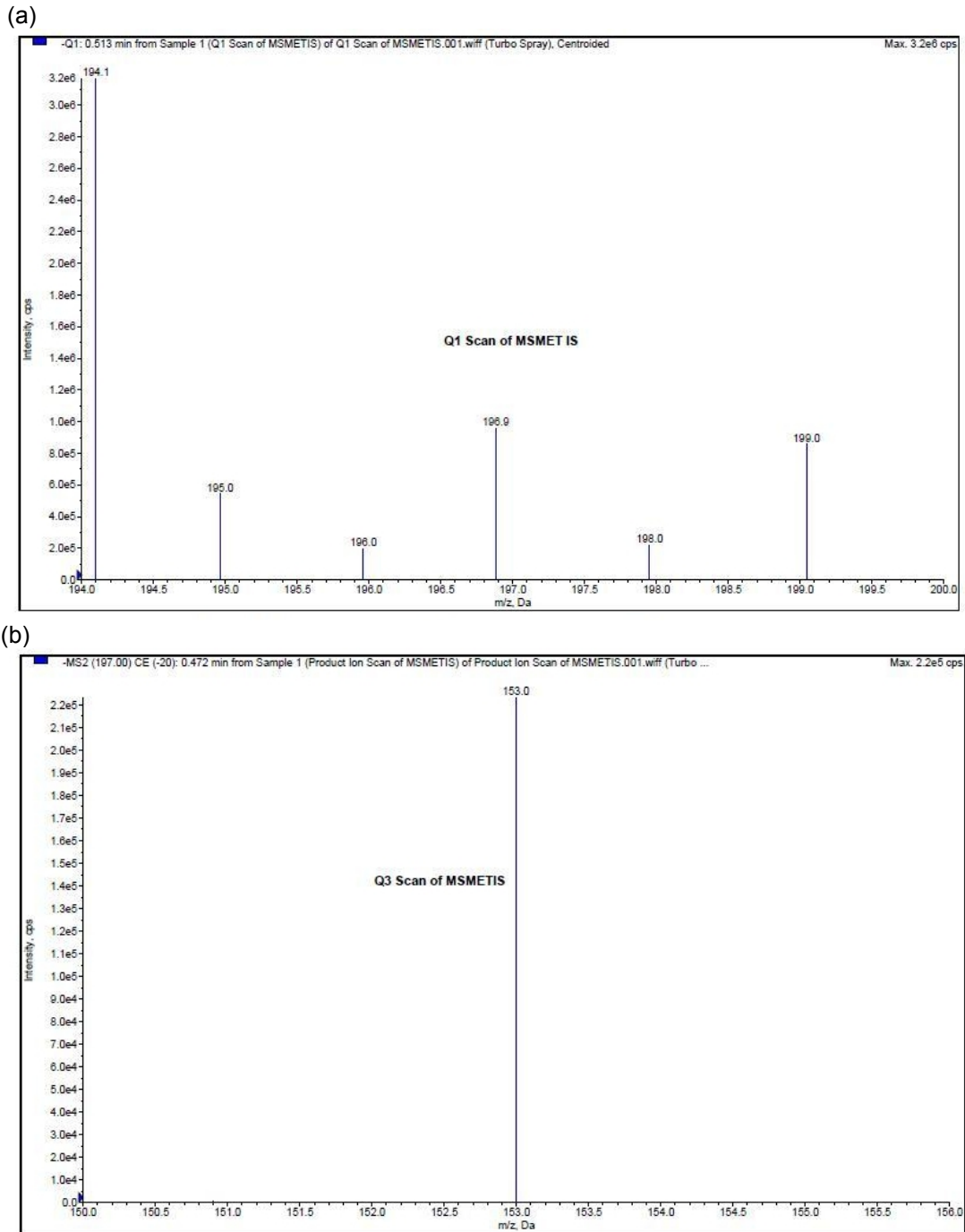
Fig. 3. Mass spectra: (a) N-Acetyl mesalamine-D3 parent ion, and (b) N-Acetyl mesalamine-D3 product ion
