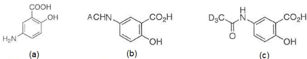
Fig. 1. Chemical structures of Mesalamine (a), N-Acetyl Mesalamine (b) and N-Acetyl Mesalamine-D3 (c)
