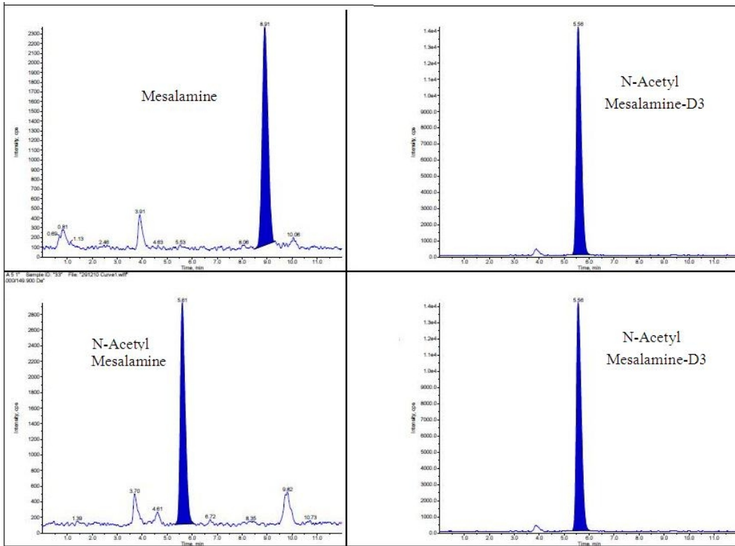
Fig. 6. Post dose chromatograms of mesalamine and N-Acetyl mesalamine at 24h
