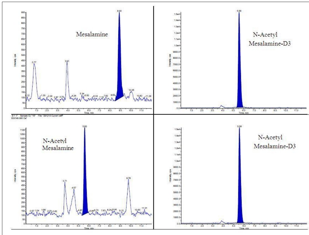
Fig. 5. LOQ Chromatograms of mesalamine and N-Acetyl mesalamine
