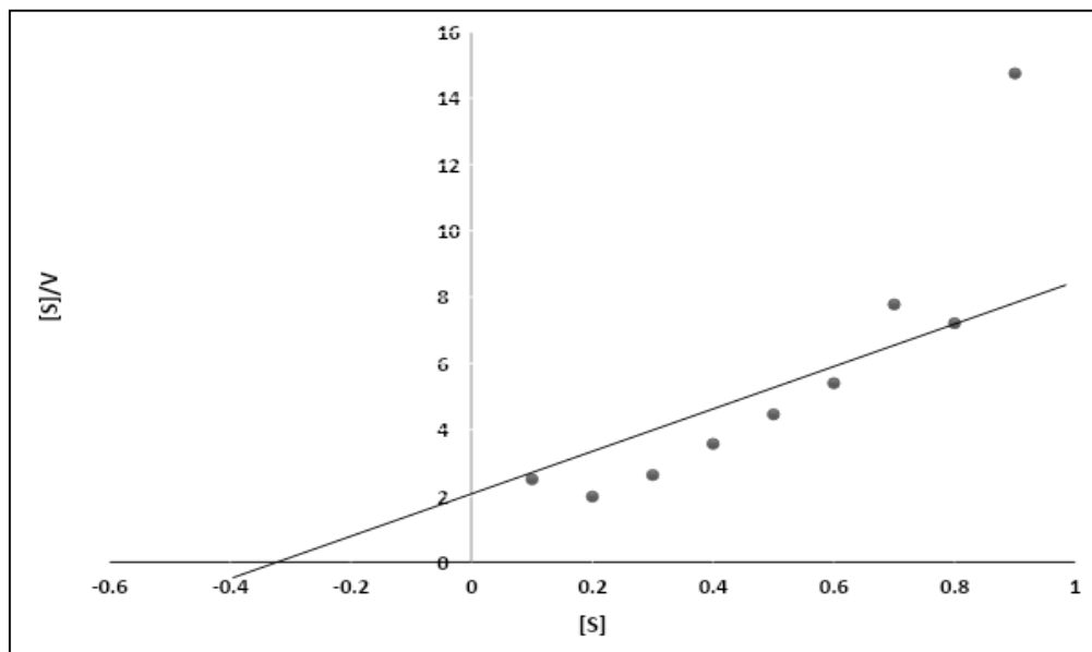
Fig. 9. Hanes-Wolf \frac{[S]}{v} against [S]
