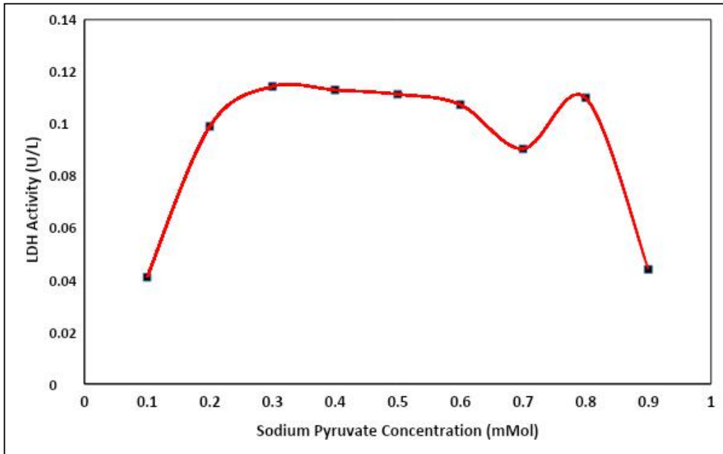
Fig. 6. Lactate dehydrogenase activity against substrate concentration using Michalis-Menten plot
