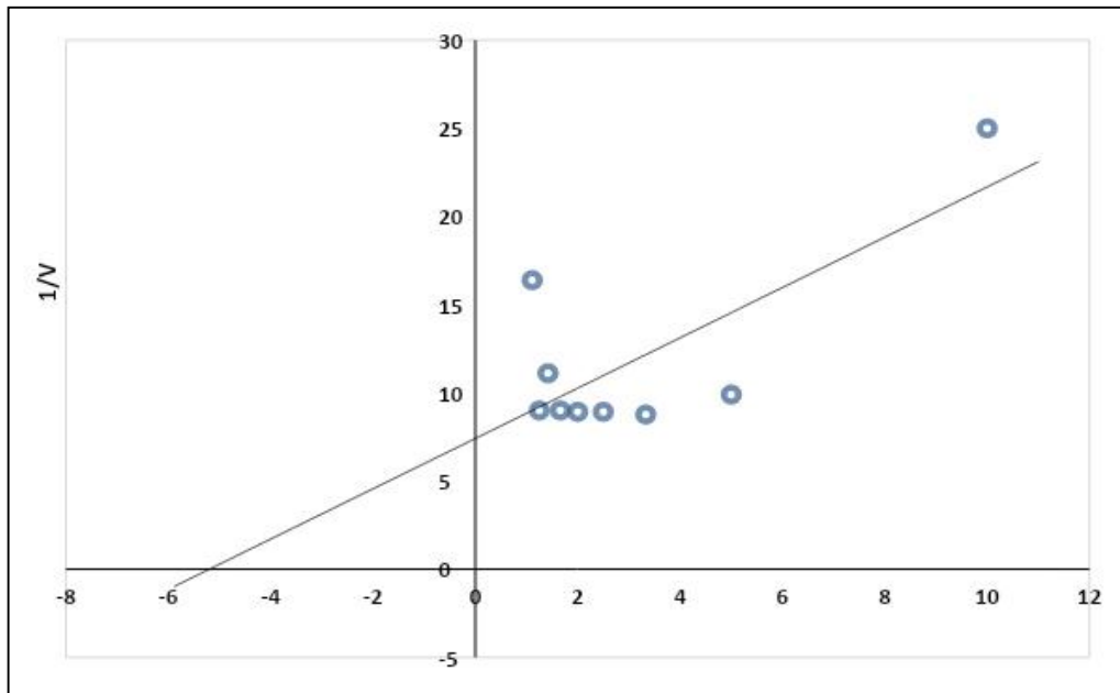
Fig. 7. Lineweaver-Burk plot of initial velocity against substrate concentration
