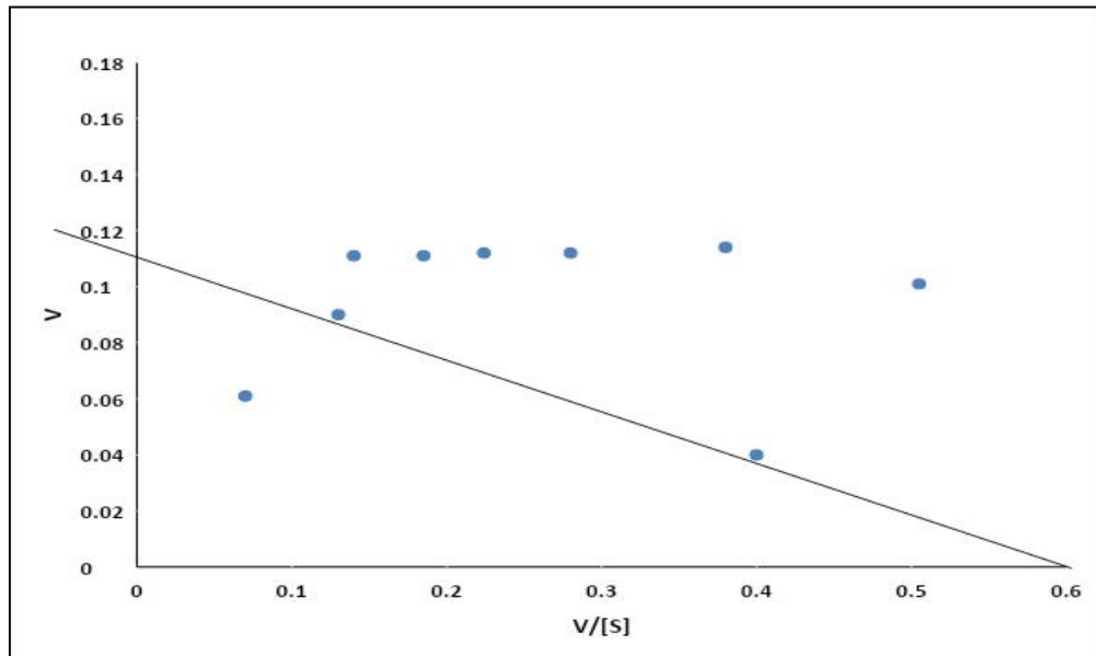
Fig. 8. Eadie-Hofstee plot of initial velocity against initial velocity divided by substrate concentration
