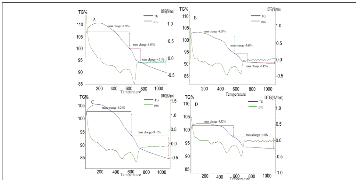
Fig.8(A-D): DTG and TG pattern of wall tile A) sample 6, B) sample 8, C) sample 9, D) sample 10.
