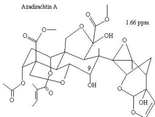
Fig. 2a. Chemical structure azadirachtin A.[3]
