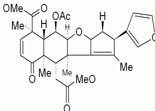
Fig 2b. Chemical structure of Nimbin [3]
