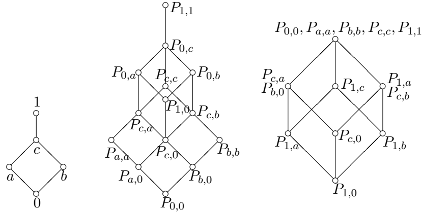
Fig. 1. Diagrams of L , A_1(L) and \text{Con}(L)
