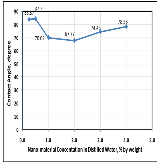
Figure 12: Contact angle Measurement by Force Tensiometer in Sandstone Formation (Si)– AUC Device.
