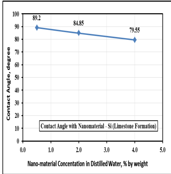
Figure 16: Contact angle Measurement by force Tensiometer in Limestone Formation (Si)- AUC Device.
