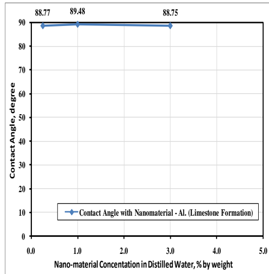
Figure 18: Contact angle Measurement by Force Tensiometer in Limestone Formation (Al)-AUC Device.
