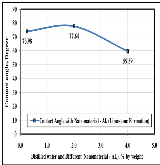
Figure 19: Contact angle Measurement by Optical Tensiometer in Limestone Formation (Al)-ENC Device
